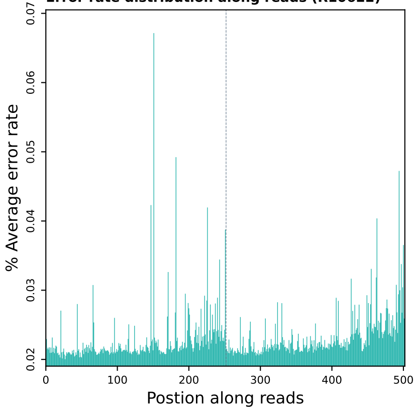
Error rate distribution along reads (R10622)
